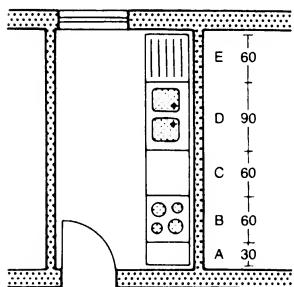
3 Effective kitchen workplace arrangement
